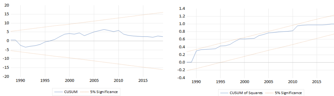
Figure 2. CUSUM 9 and CUSUMSQ 10 Tests
