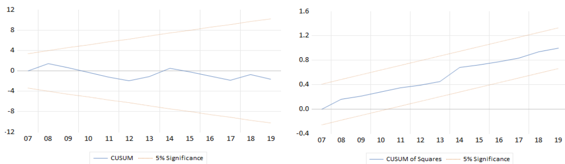
Figure 1. CUSUM 9 and CUSUMSQ 10 Tests
