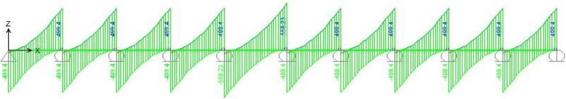
Figure 5. Crane Girder Shear Force Diagram (kN)
